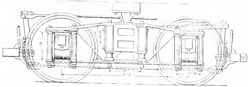
Fig. 4792. Side Elevation.
